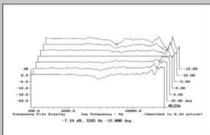
Fig.6 Canton Reference 5, vertical response family at 1m, normalized to response on optimal axis, from back to front: differences in response 15°–5° above axis, reference response, differences in response 5°–15° below axis.
