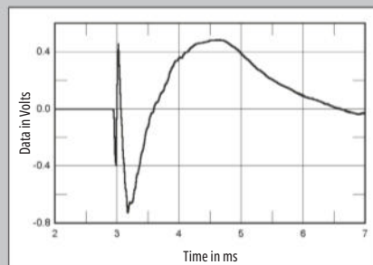
Fig.7 Canton Reference 5, step response on optimal axis at 1m (5ms time window, 30kHz bandwidth).
