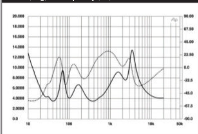
Fig.1 Canton Reference 5, electrical impedance (solid) and phase (dashed) (2 ohms/vertical div.).
