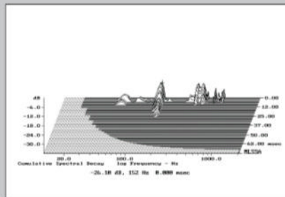
Fig.2 Canton Reference 5, cumulative spectral-decay plot calculated from output of accelerometer fastened to center of a sidewall level with the lower woofer (measurement bandwidth, 2kHz).
