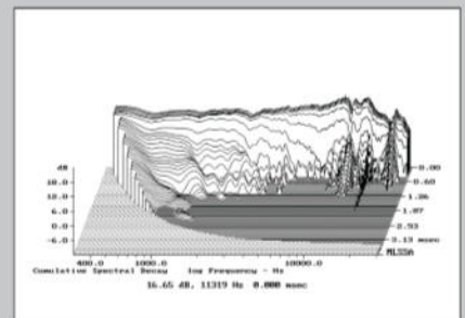
Fig.8 Canton Reference 5, cumulative spectral-decay plot on optimal axis at 1m (0.15ms risetime).
