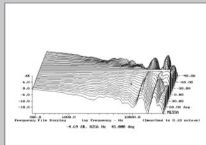
Fig.5 Canton Reference 5, lateral response family at 1m, normalized to response on optimal axis, from back to front: differences in response 90°-5° off axis, reference response, differences in response 5°-90° off axis.
