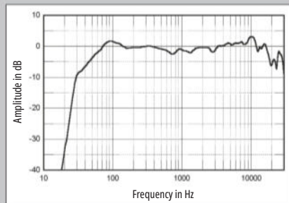
Fig.4 Canton Reference 5, anechoic response on optimal axis at 1m, averaged across 30° horizontal window and corrected for microphone response, with the complex sum of the nearfield responses plotted below 300Hz.
